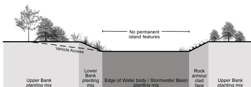
Figure 17: Typical Basin Section
