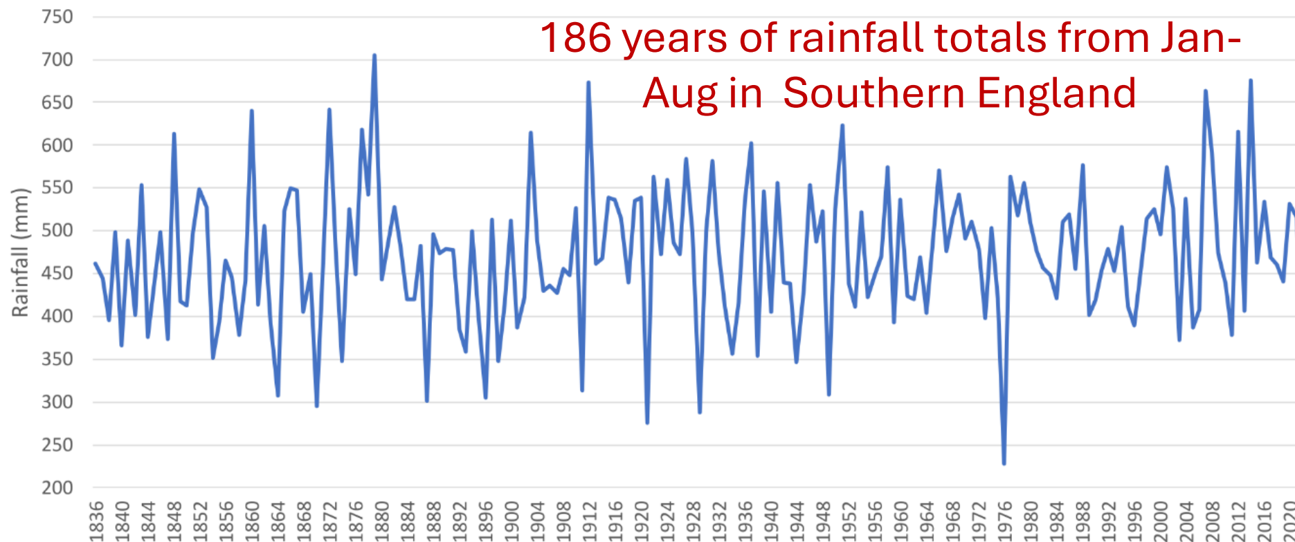
FIGURE 78 Southern England rainfall totals January–August 1836–2022.
