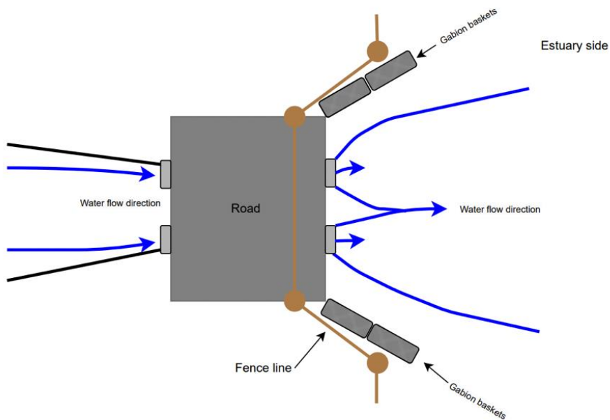
Figure 15. Double culvert design at estuary edge.
