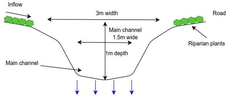
Figure 11. Swale design. Swales have a shallow, curved shape, allowing for a wider width to be covered at the top. Improving water infiltration into the soil and controlling water quality and sediment runoff.
